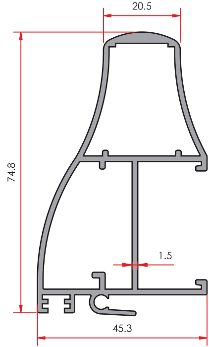
REINFORCEMENT WING TAKVİYELİ KANAT
