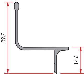
FLYSWATER RAIL SİNEKLİK RAYI
